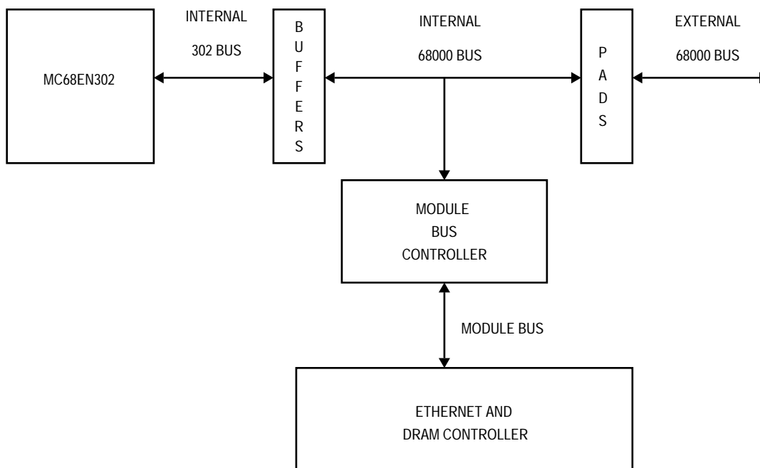
Figure 3. BusStructure
