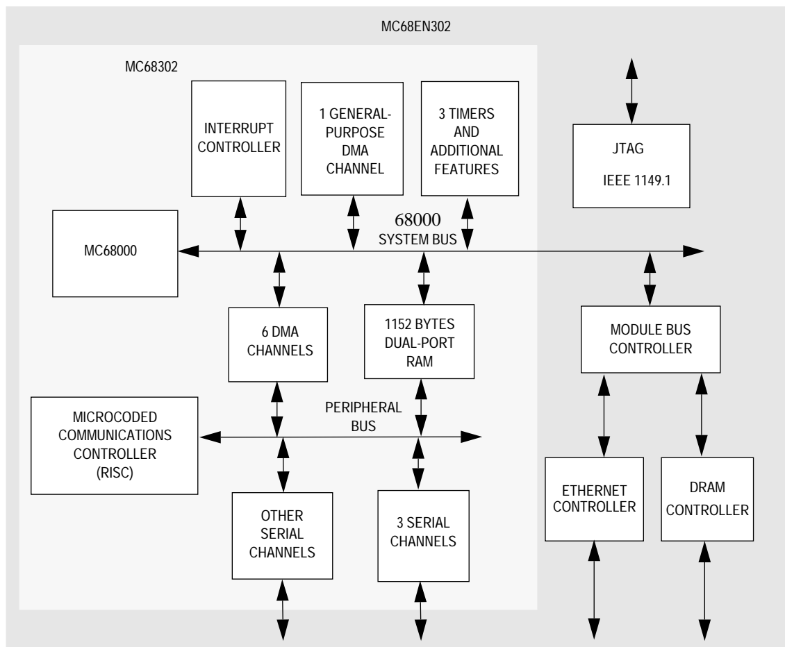
Figure 1. MC68EN302 Block Diagram
