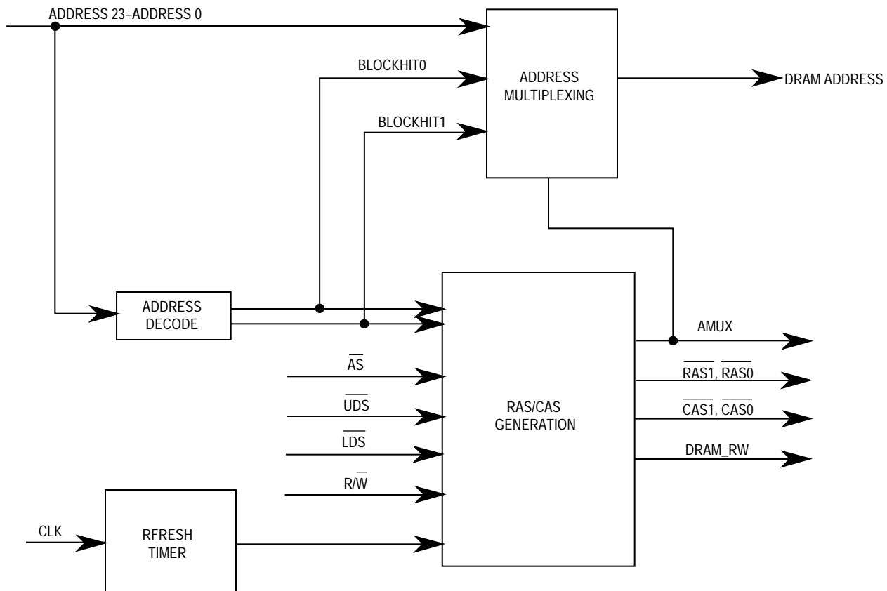
Figure 4. DRAM Controller
