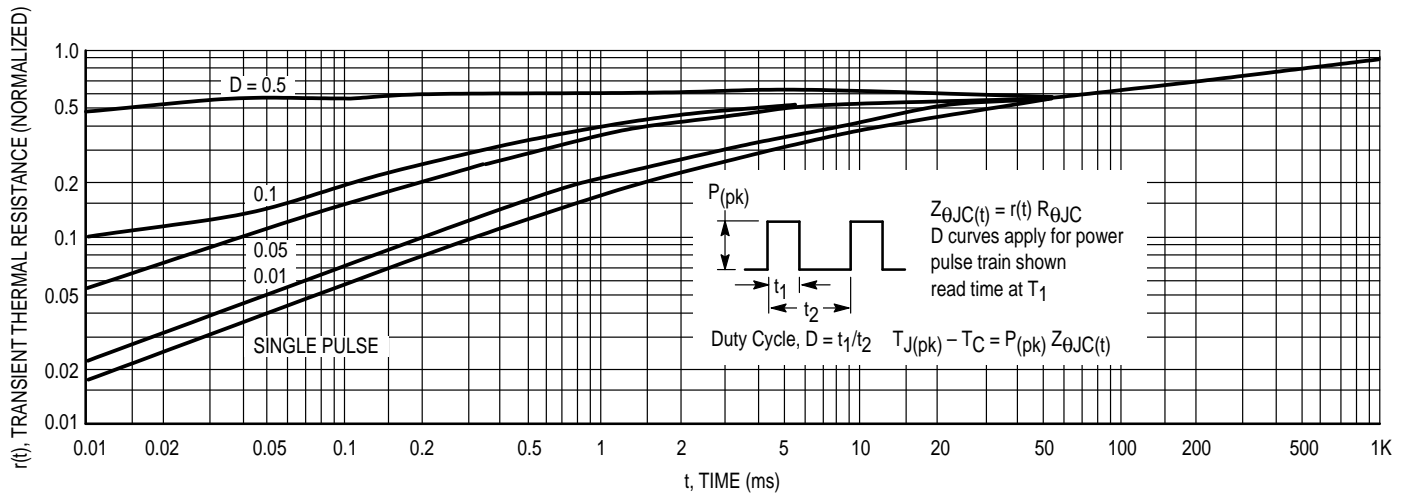
Figure 5. Thermal Response
