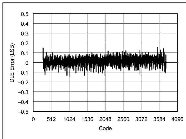
FIGURE 2. ADC774 Board DLE with Improved Ground.
