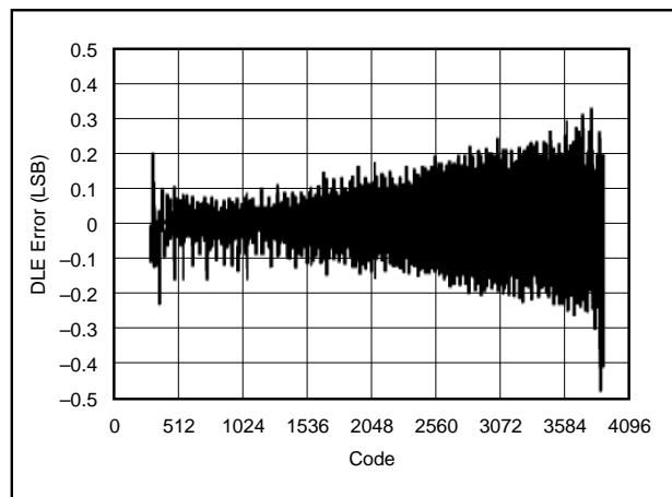
FIGURE 1. ADC774 Board DLE with Poor Ground.
