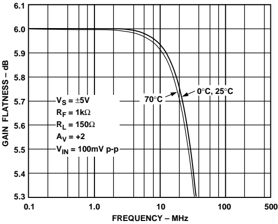
Figure 7. 0.1 dB Flatness vs. Frequency Over Temperature; V_S = \pm 5V
