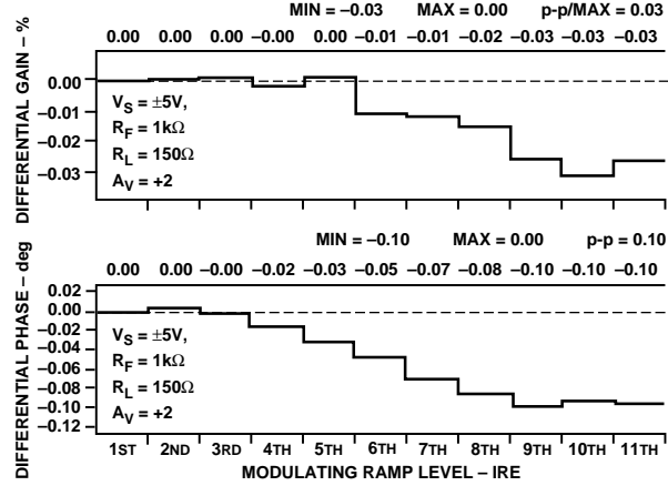
Figure 9. Differential Gain and Phase, V_S = \pm 5V
