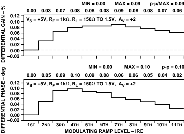
Figure 8. Differential Gain and Phase, V_S = +5V
